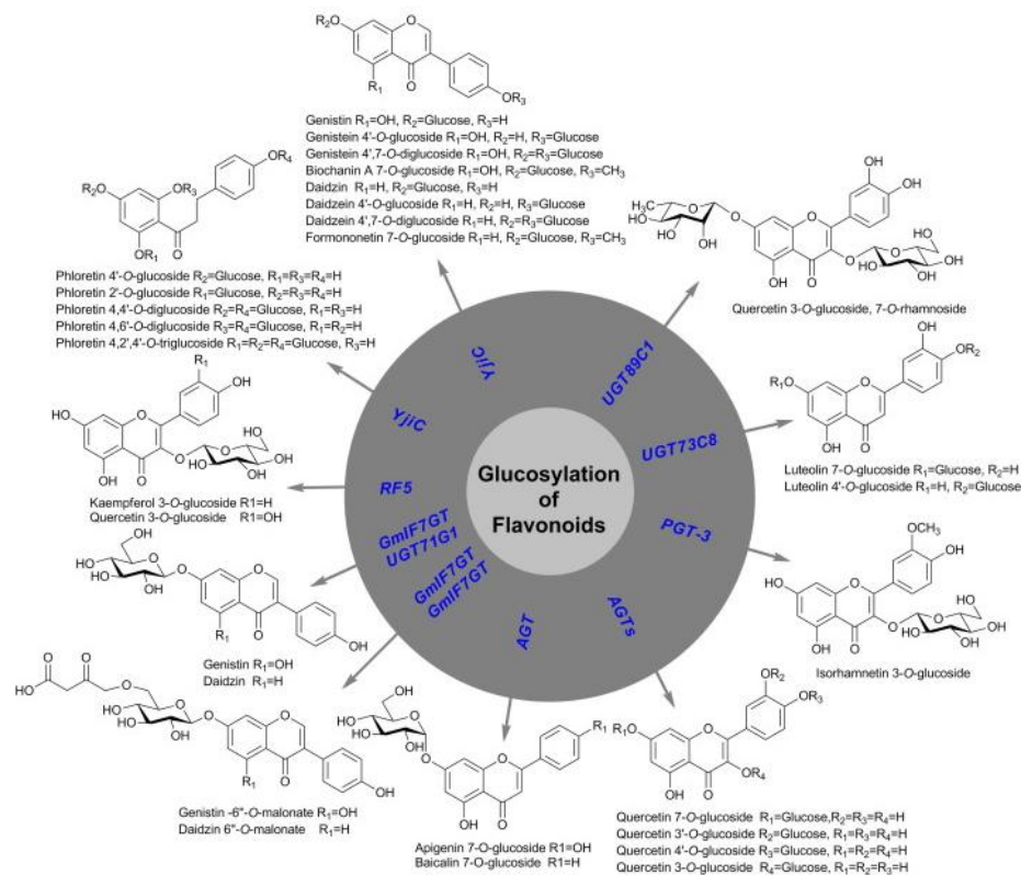
Figure 2: Glycosylation of Flavonoids
