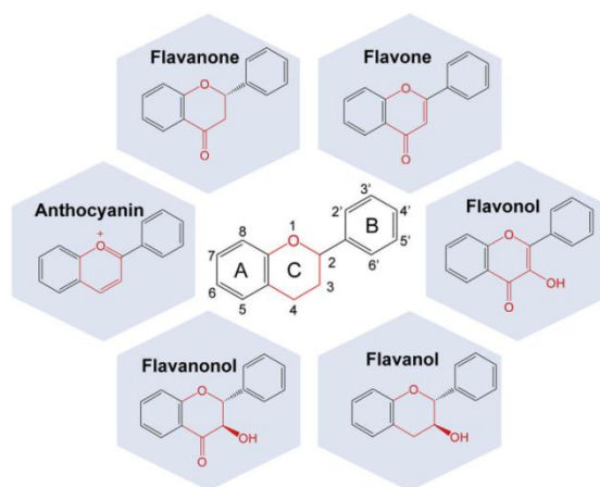
Figure 3: Flavonoid Major Classes
