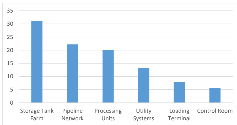
Figure 3: Graphical Representation of the percentage of Vulnerable Refinery Sections Affected by Multi-Hazards
